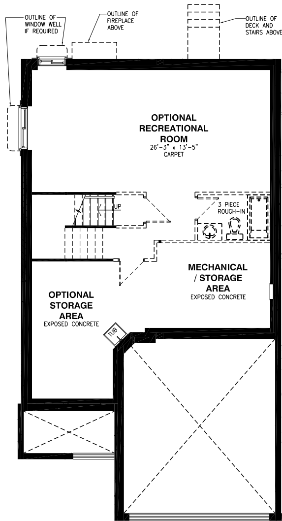
Basement Floor
