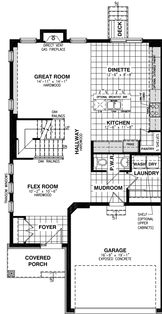
Ground Floor
