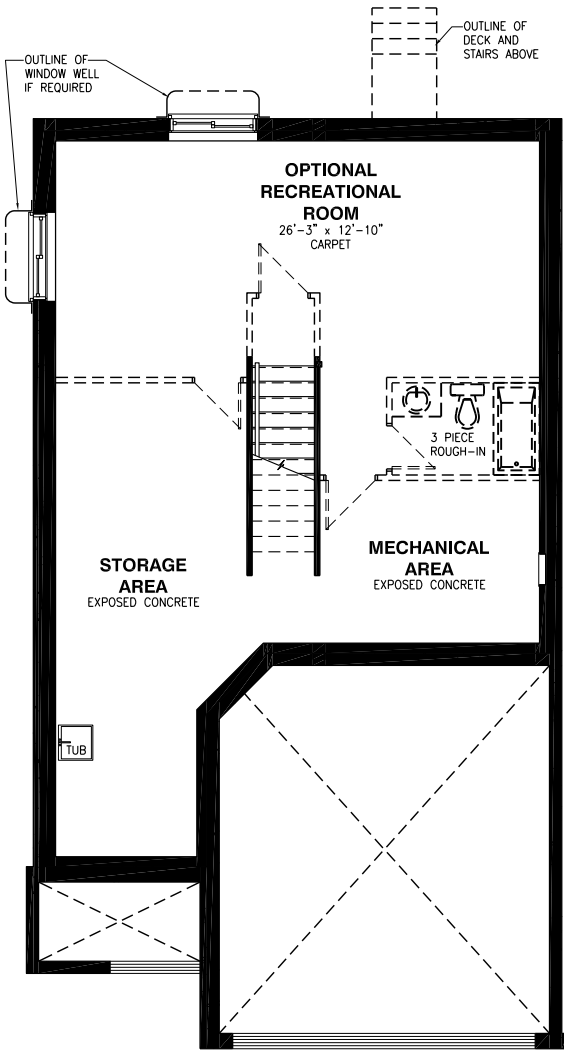
Basement Floor
