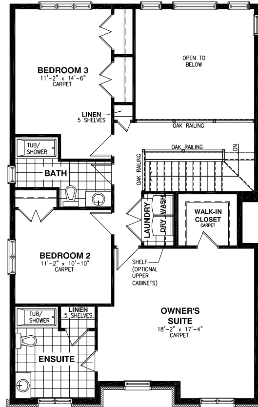
Second Floor - 3 Bedroom - Elevation A
