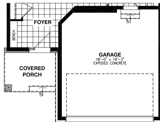
Ground Floor - Elevation B
