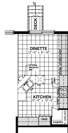
Optional Kitchen #1
