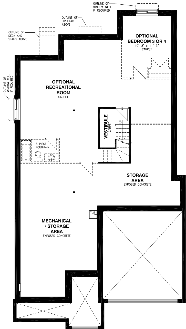
Basement Floor - Elevation A
