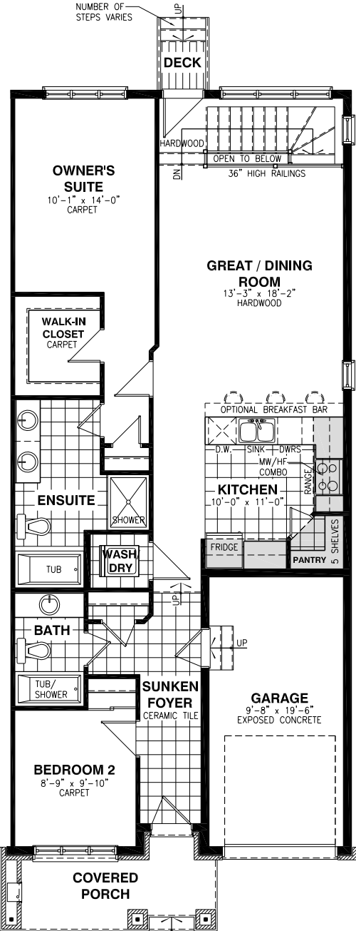
GROUND FLOOR PLAN STANDARD 2 BEDROOM
