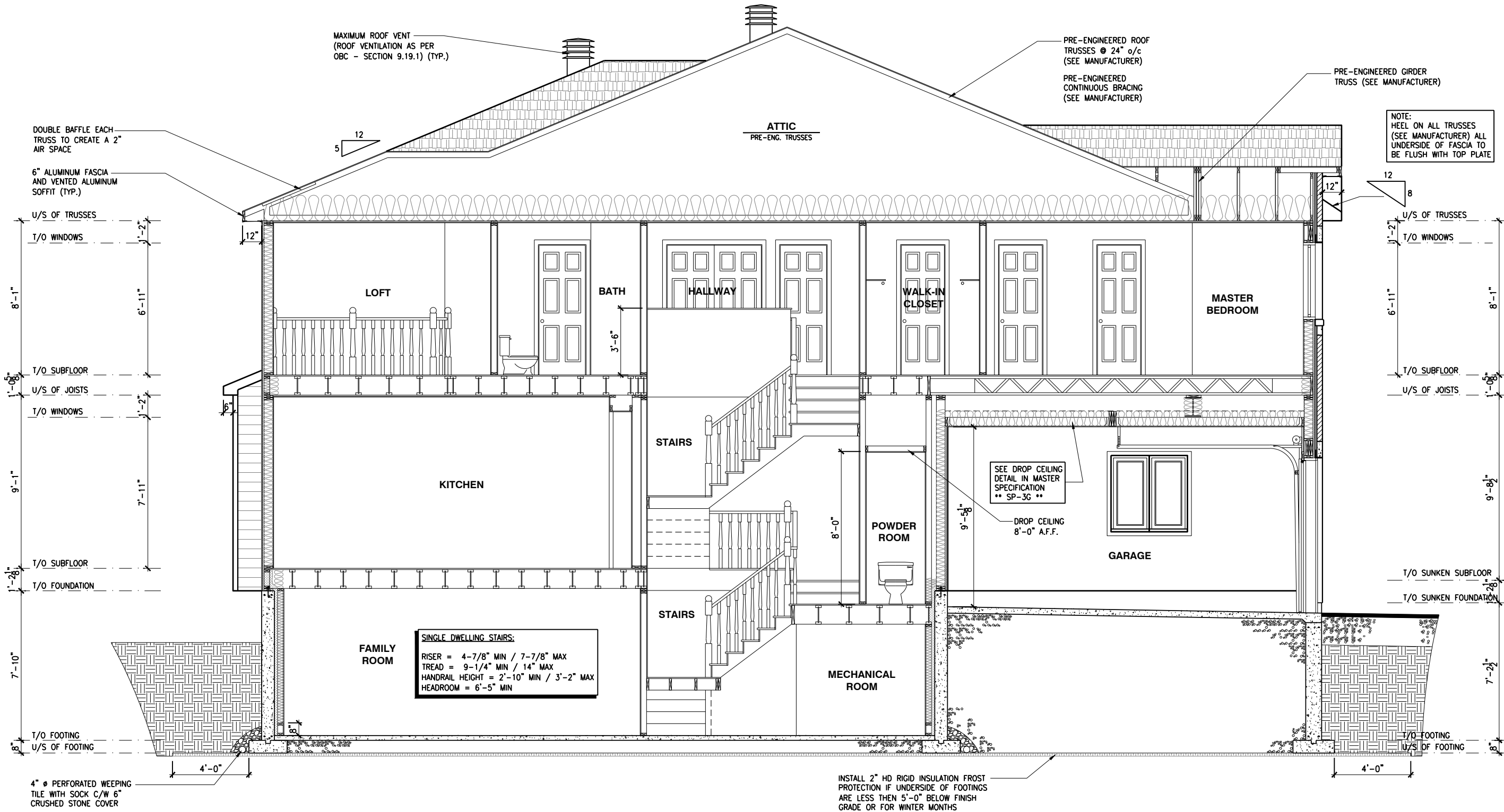
1 BUILDING SECTION A.3a SCALE: 3/16" = 1'-0"
