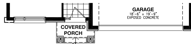
Ground Floor - Elevation B
