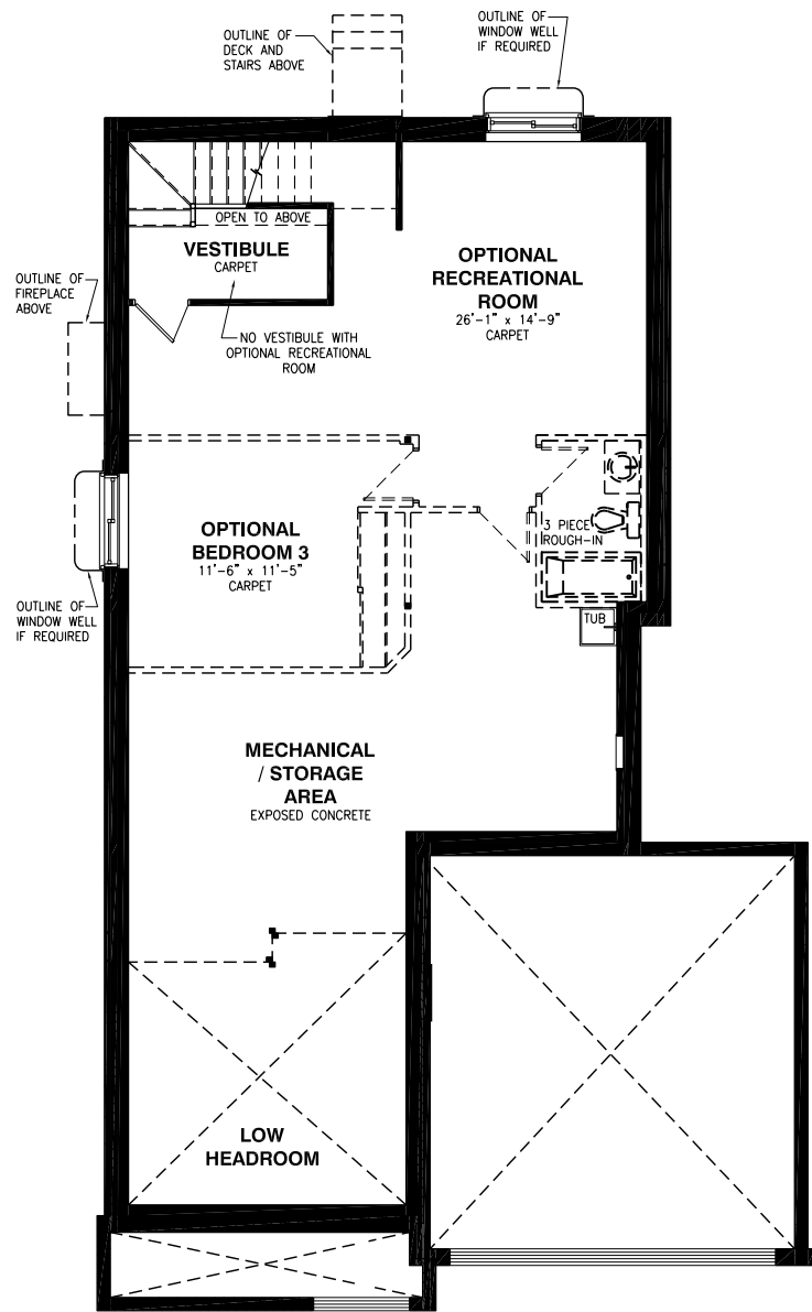
Basement Floor - Elevation A
