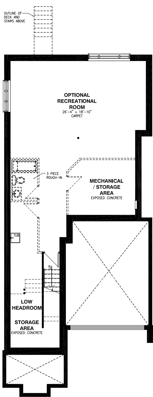
Basement Floor - Elevation A
