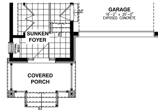
Ground Floor - Elevation B
