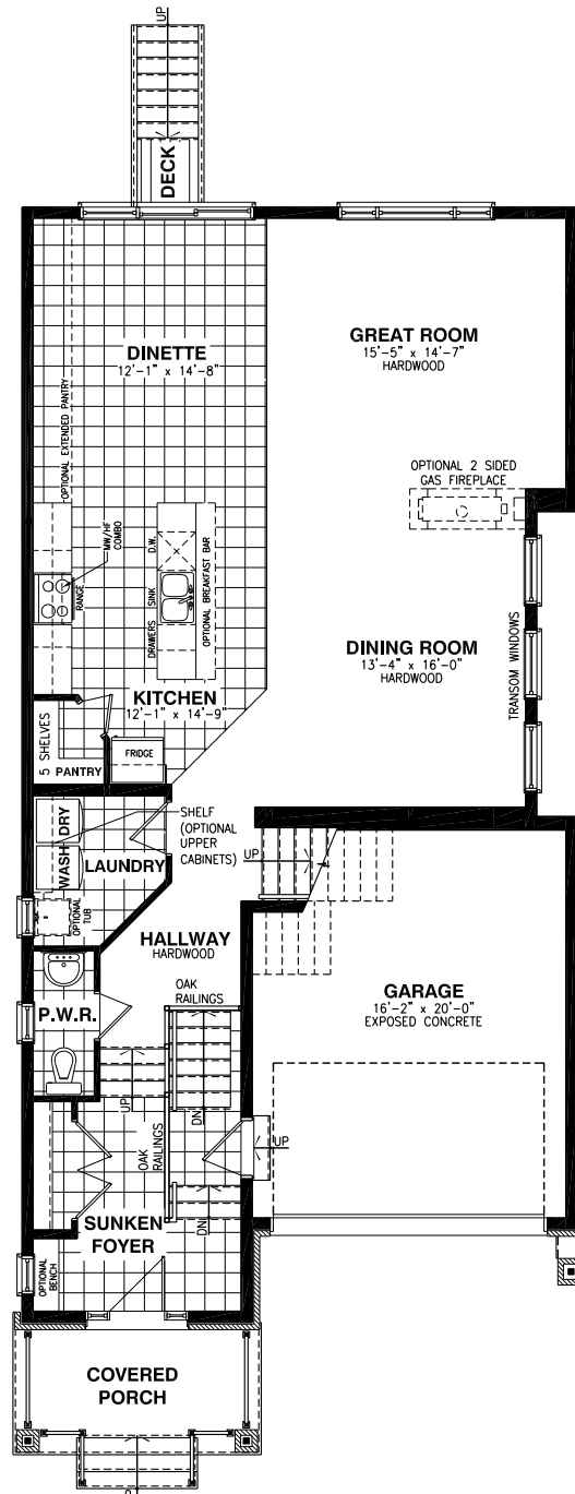
Ground Floor - Elevation A
