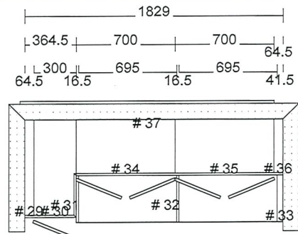
OPT LAUNDRY 914mm UPPERS INSTALL CABS 1479mm FROM FINISHED FLOOR
