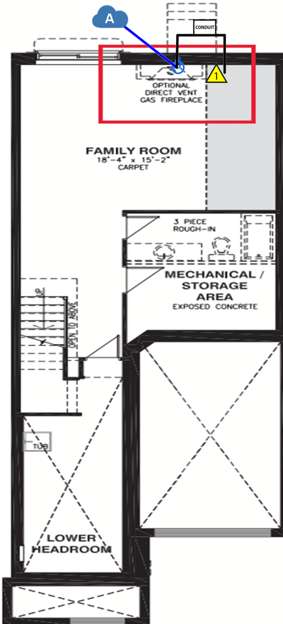
BASEMENT FLOOR
