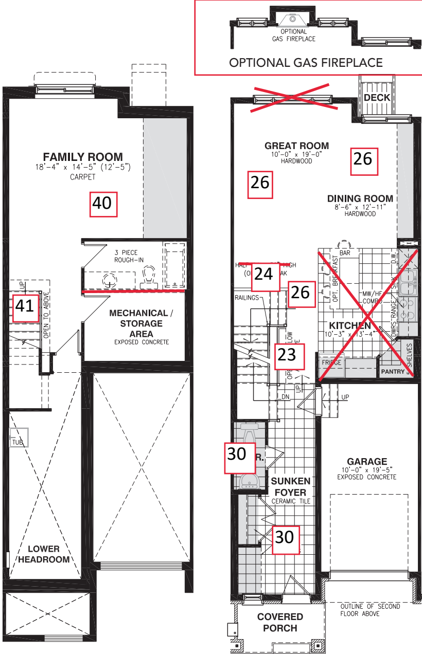
BASEMENT FLOOR
