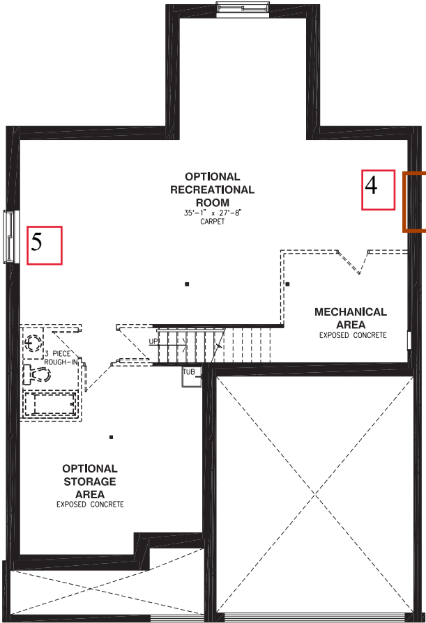
BASEMENT FLOOR
