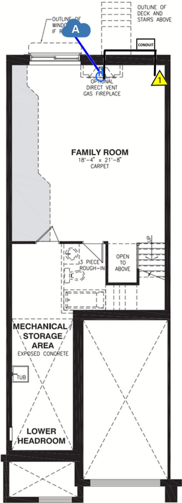
BASEMENT FLOOR
