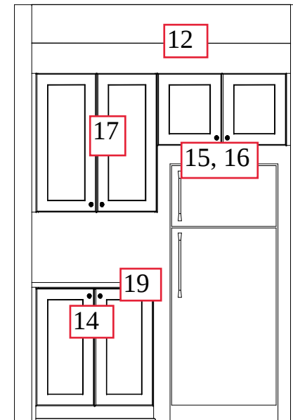
#11 - Optional Kitchen Layout #1
