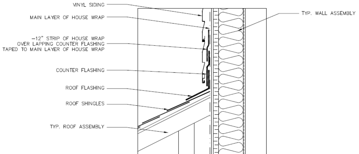
1 SP-23 1'-1/2" = 1'-0" ROOF FLASHING - VINYL SIDING
