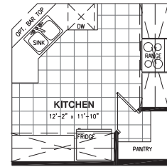
OPTIONAL KITCHEN LAYOUT
