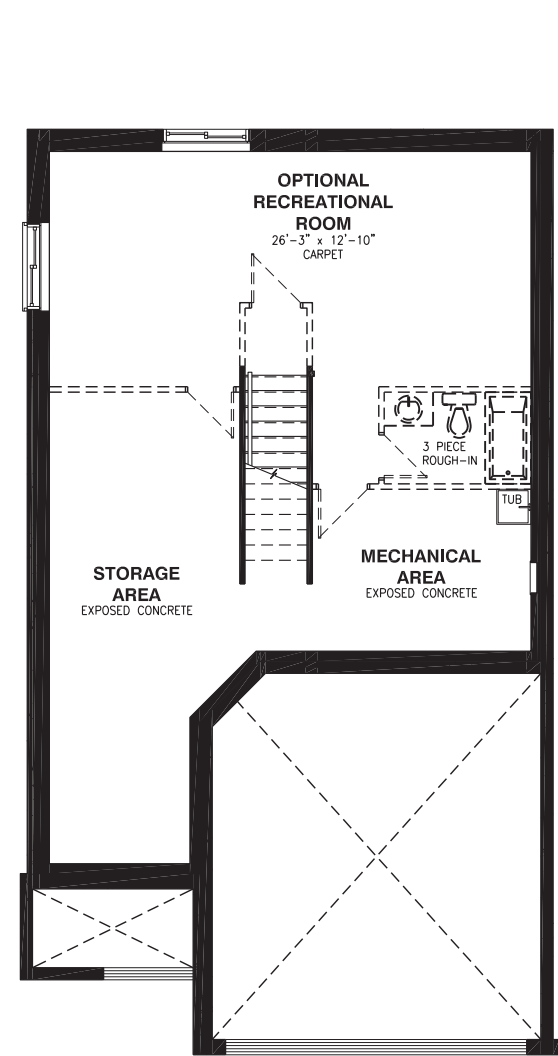
BASEMENT FLOOR
