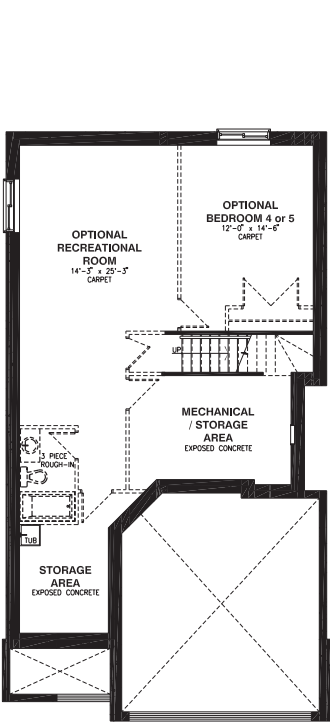
BASEMENT FLOOR
