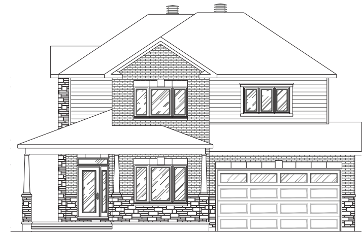
ELEVATION CORNER LOT
