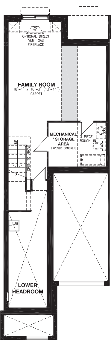
BASEMENT FLOOR
