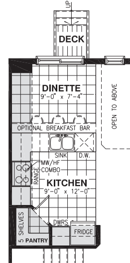
OPTIONAL KITCHEN #2
