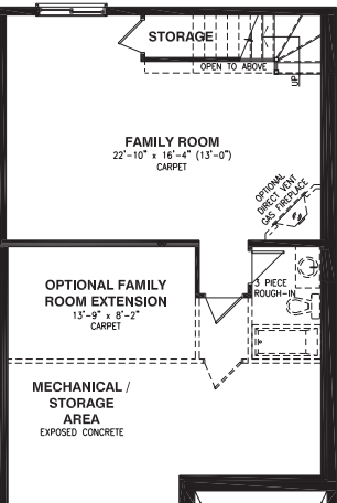
WALKOUT BASEMENT GARAGE END WHERE APPLICABLE
