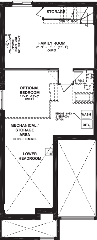
BASEMENT FLOOR PORCH END
