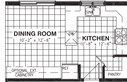
OPTIONAL KITCHEN #1
