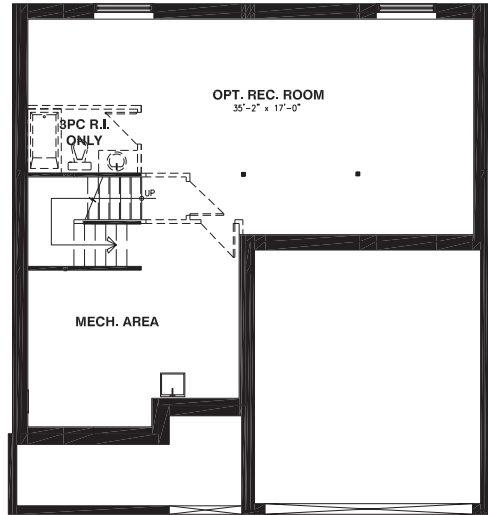
BASEMENT FLOOR
