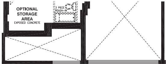
BASEMENT FLOOR - ELEVATION B
