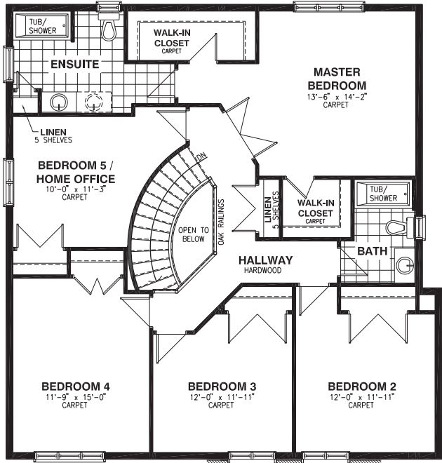
SECOND FLOOR - ELEVATION A
