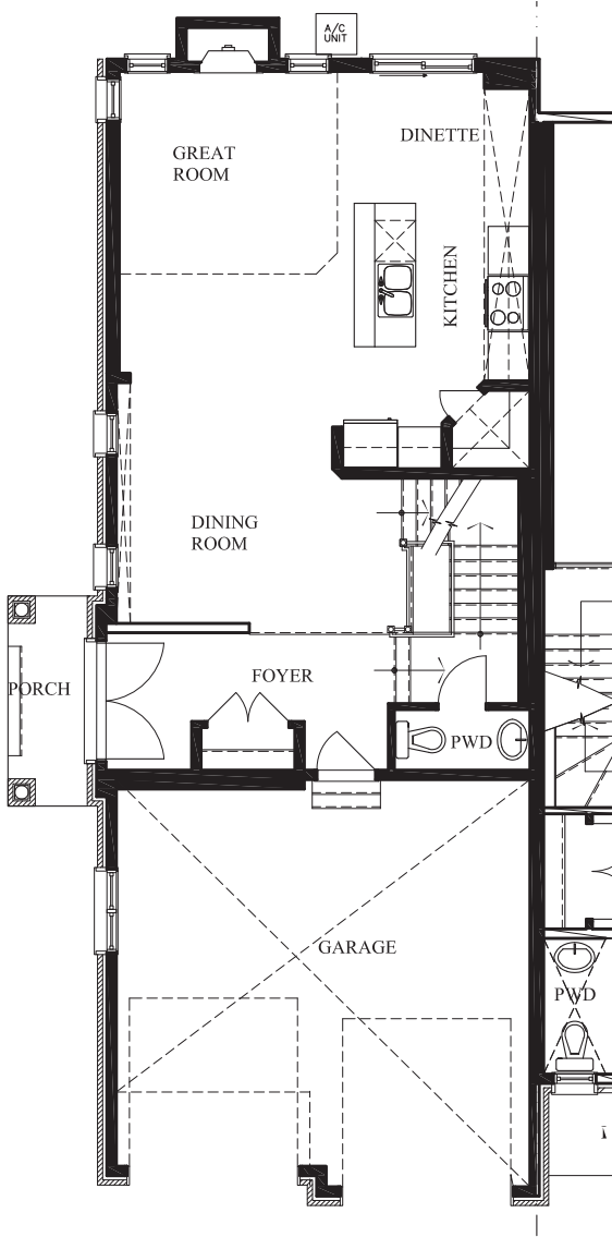
743.14 sq.ft. GROUND FLOOR
