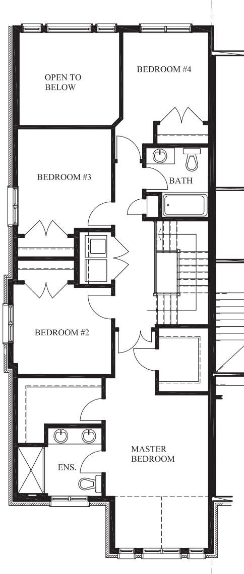
936.5sq.ft SECOND FLOOR
