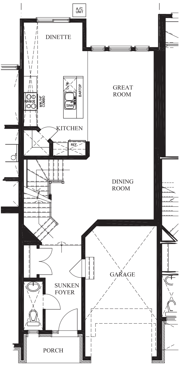
767.30 GROUND FLOOR
