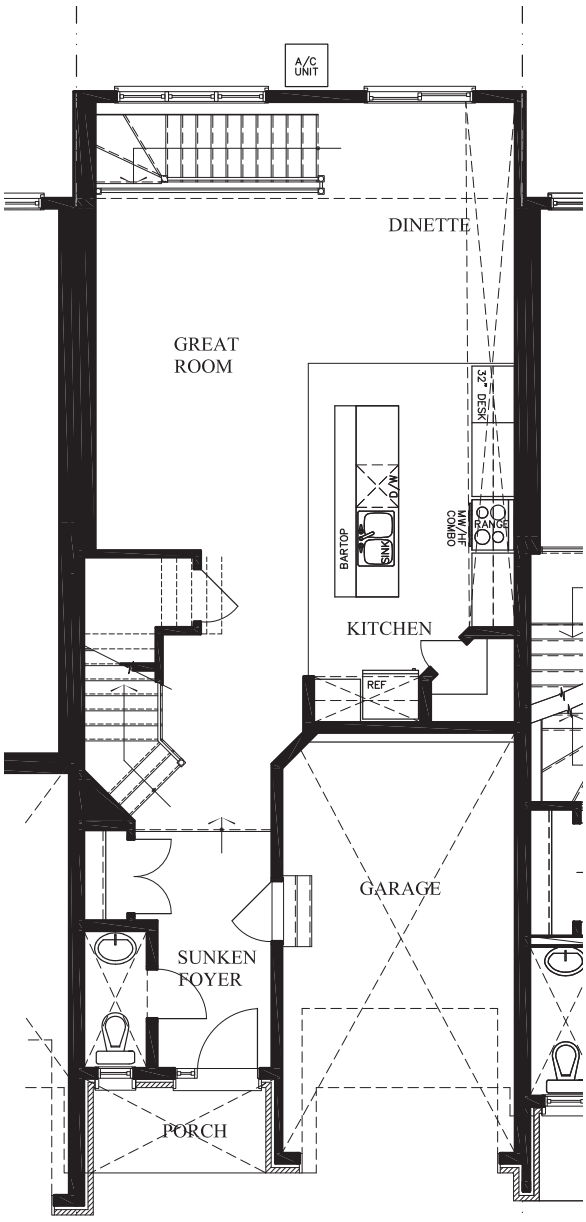
742.64 GROUND FLOOR
