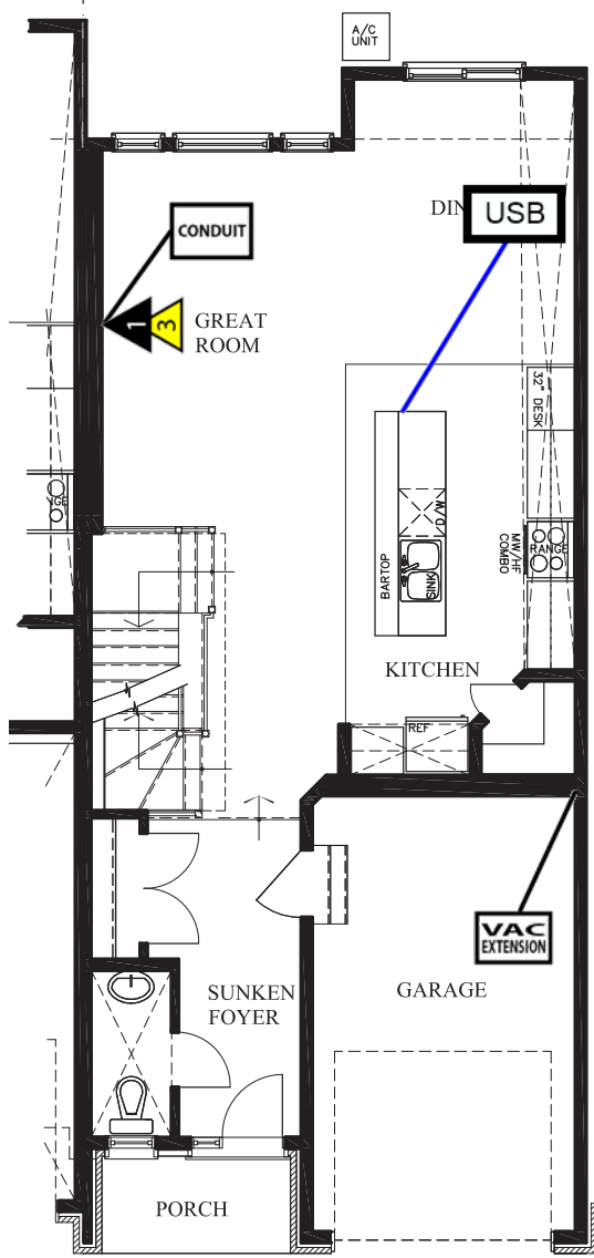
765 06 GROUND FLOOR
