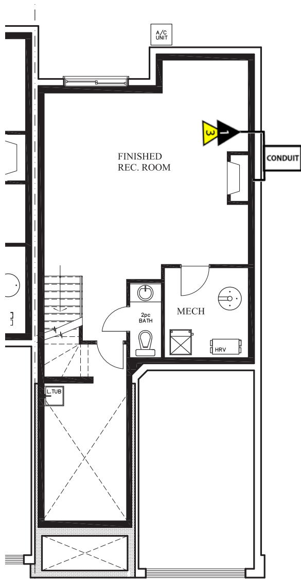
478.36 sq.ft. fin bsmt BASEMENT FLOOR
