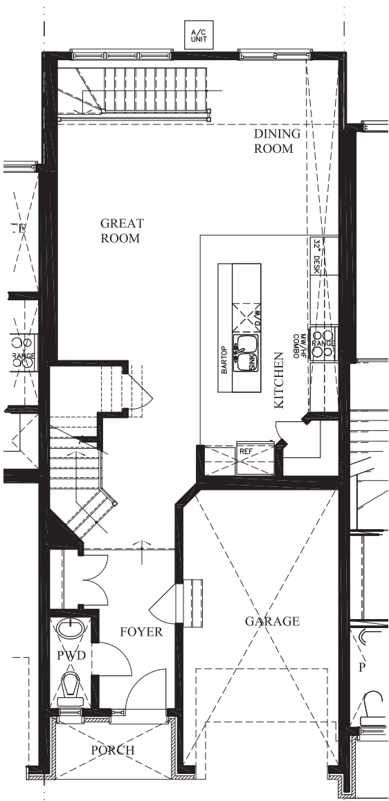
742.64 sq.ft. GROUND FLOOR
