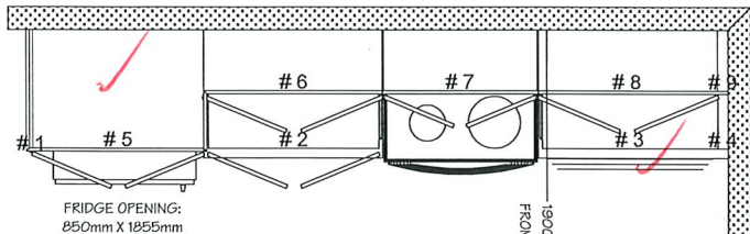
KITCHEN 1067mm UPPERS
