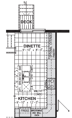
OPTIONAL KITCHEN #3
