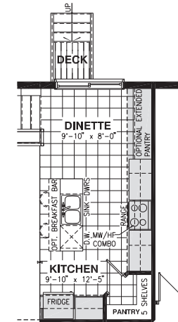
OPTIONAL KITCHEN #1
