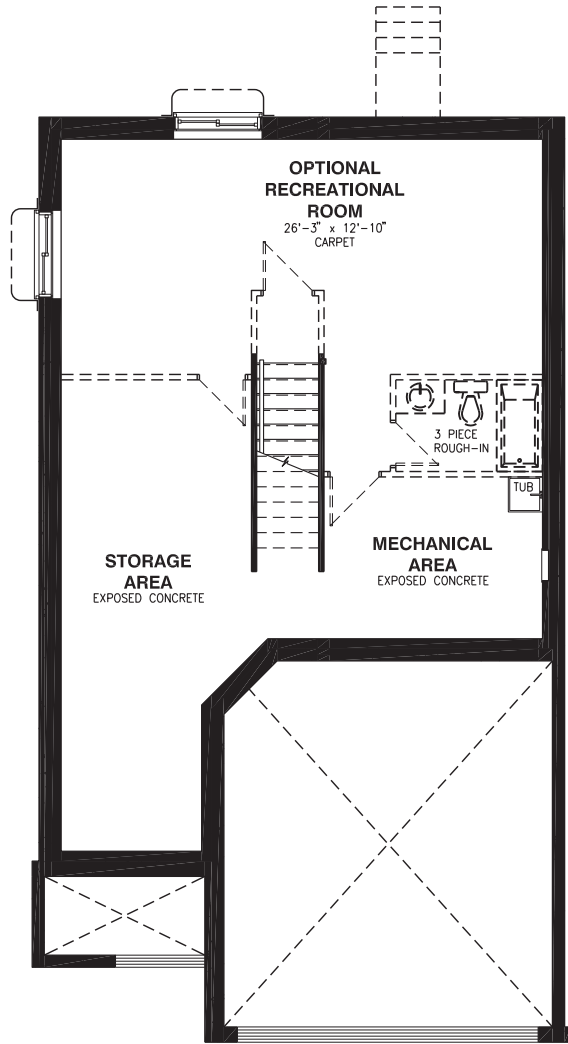
BASEMENT FLOOR
