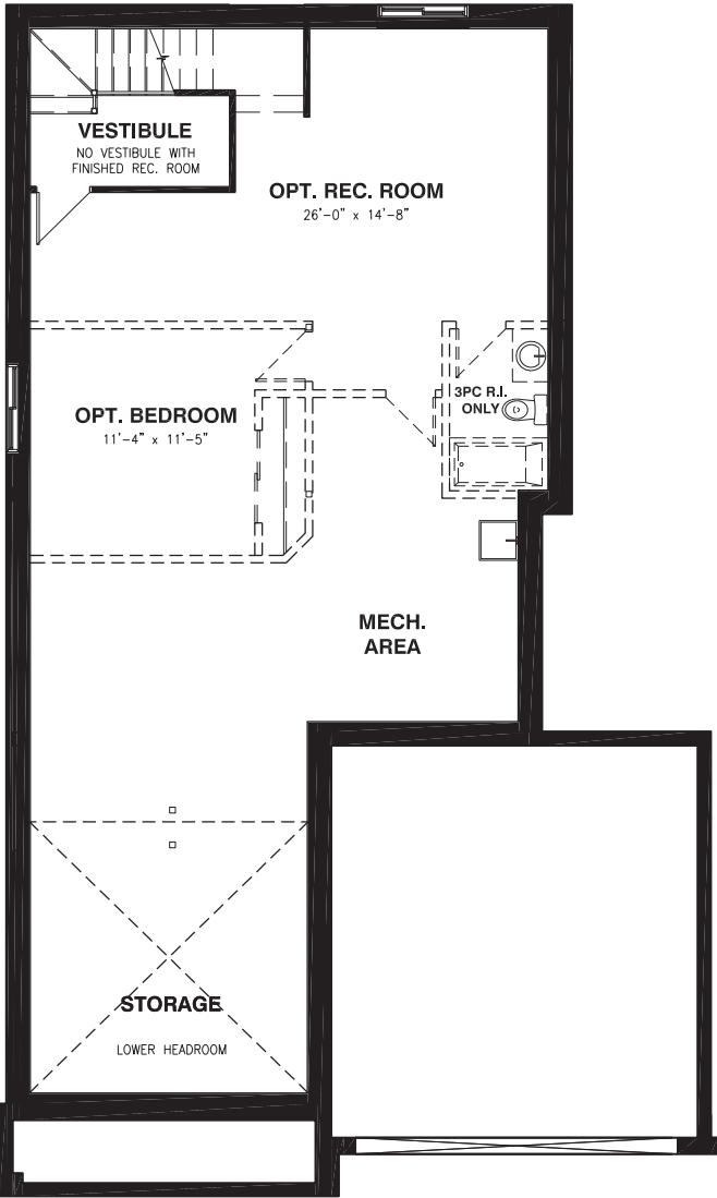
BASEMENT FLOOR A
