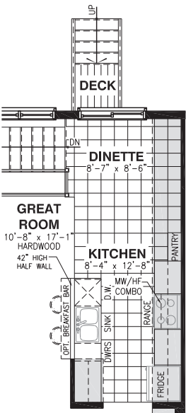
OPTIONAL KITCHEN #1
