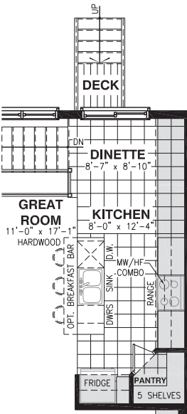
OPTIONAL KITCHEN #2
