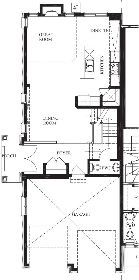
743.14 sq.ft. GROUND FLOOR
