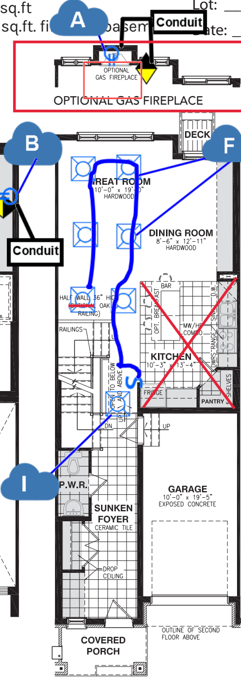
GROUND FLOOR
