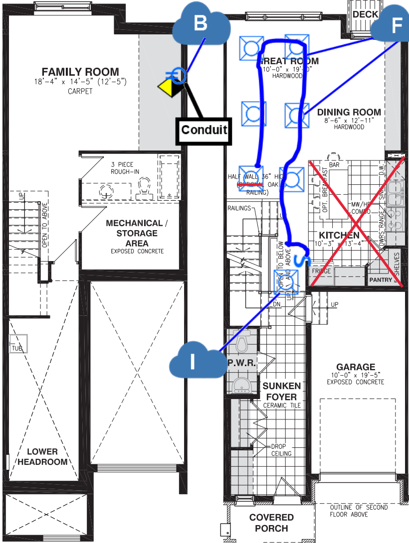
BASEMENT FLOOR
