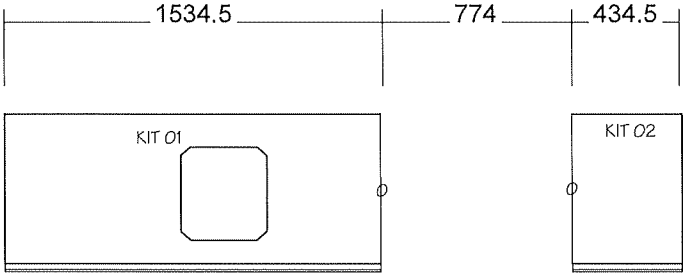
KITCHEN COLOUR (A) RK7002T
