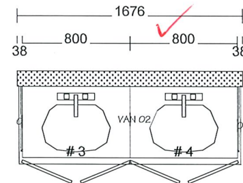
OPT. 5PC ENSUITE 2ND FLOOR
