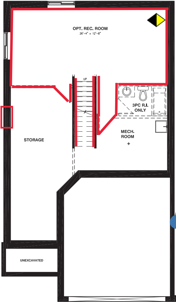
BASEMENT FLOOR
