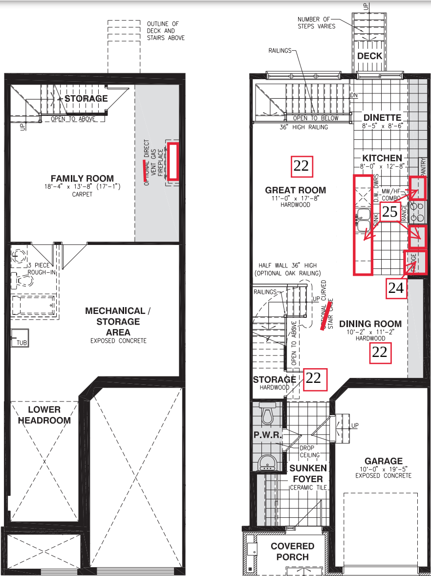
BASEMENT FLOOR
