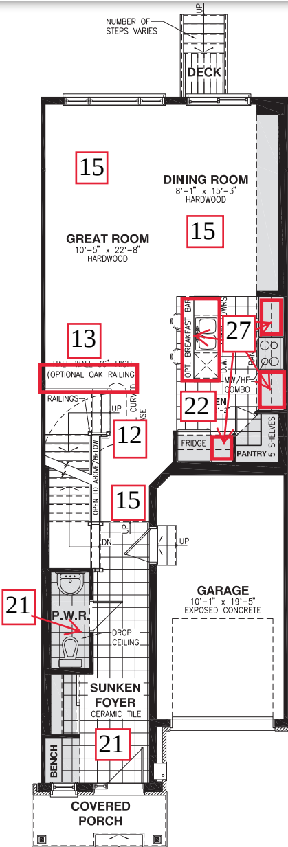
GROUND FLOOR
