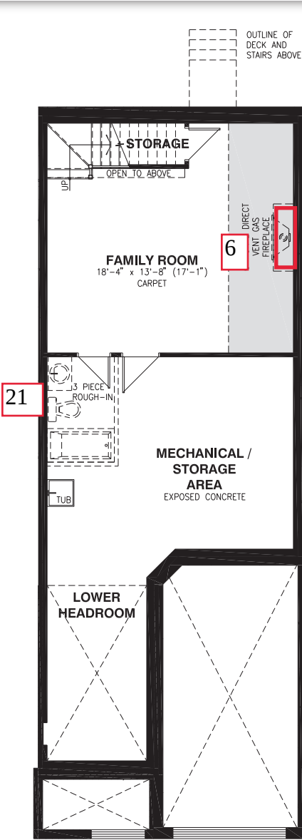
BASEMENT FLOOR
