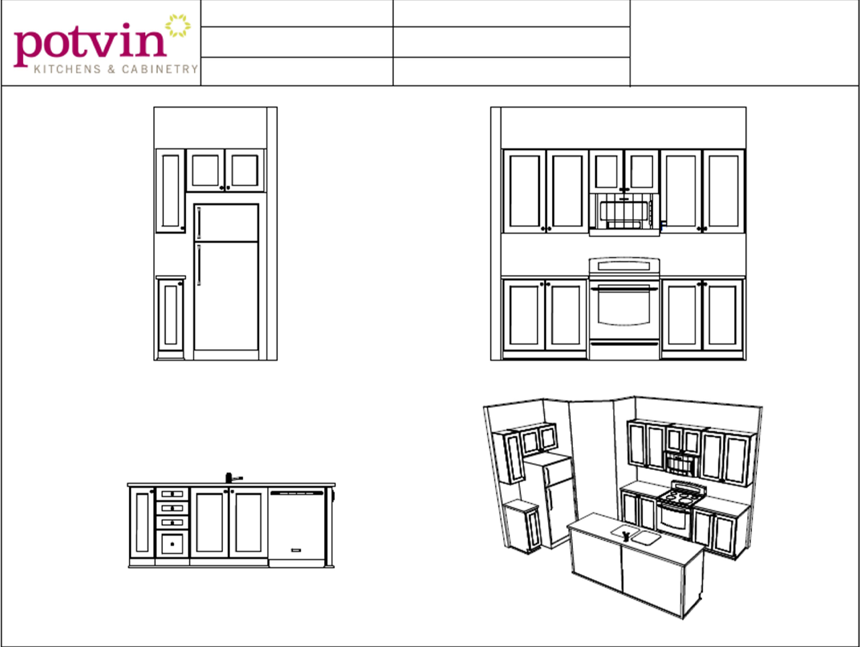
- STANDARD KITCHEN LAYOUT
