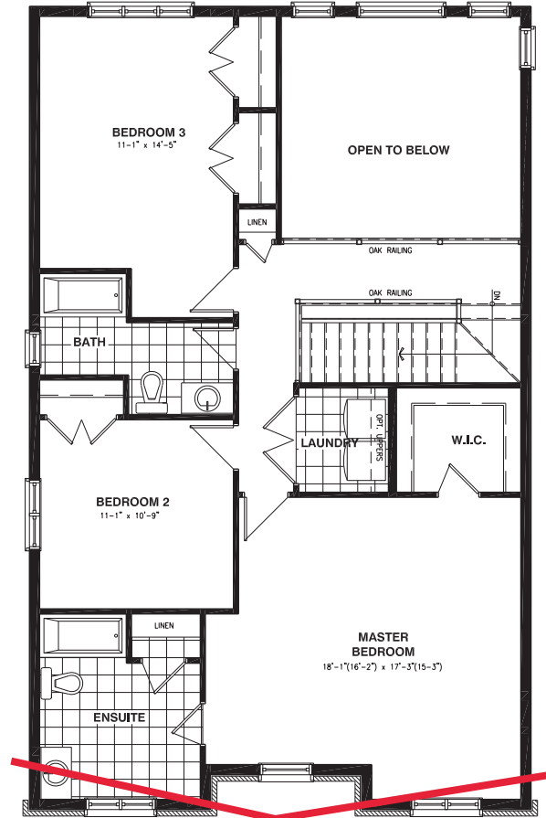
SECOND FLOOR - 3 BEDROOMS - ELEVATION A
