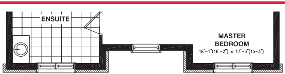
SECOND FLOOR - 3 & 4 BEDROOMS - ELEVATION B
