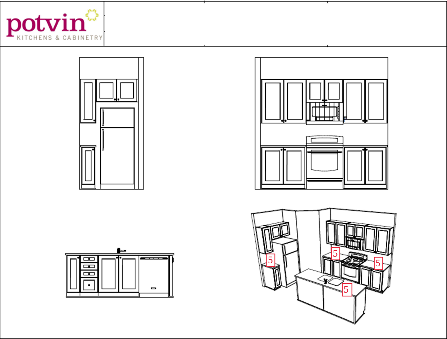
STANDARD KITCHEN LAYOUT – MODEL #826 BRADLEY
