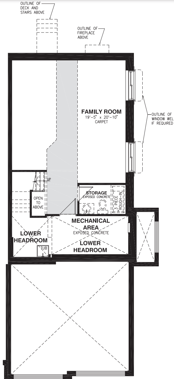
BASEMENT FLOOR
