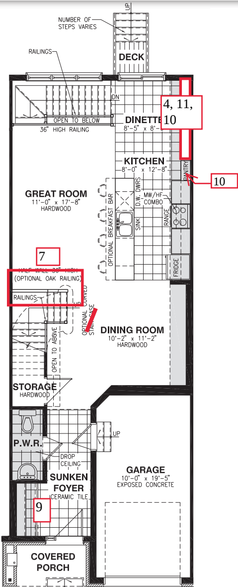
GROUND FLOOR
